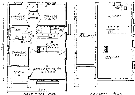
Plan for Above Six Bungalows.
