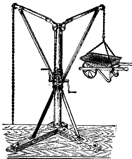
Height 7 feet. Swing full circle. Capacity 800 lbs.
