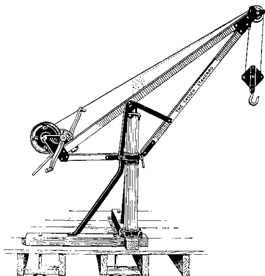
Height 8 feet. Swing 12 feet. Capacity 2500 lbs.
