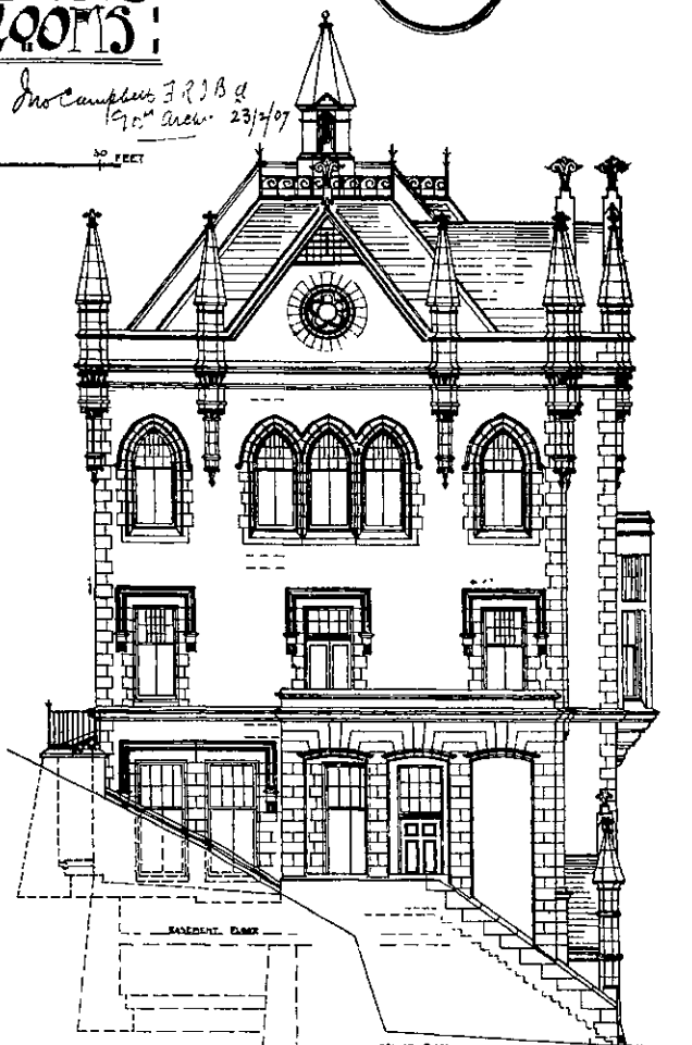
WEST ELEVATION.
