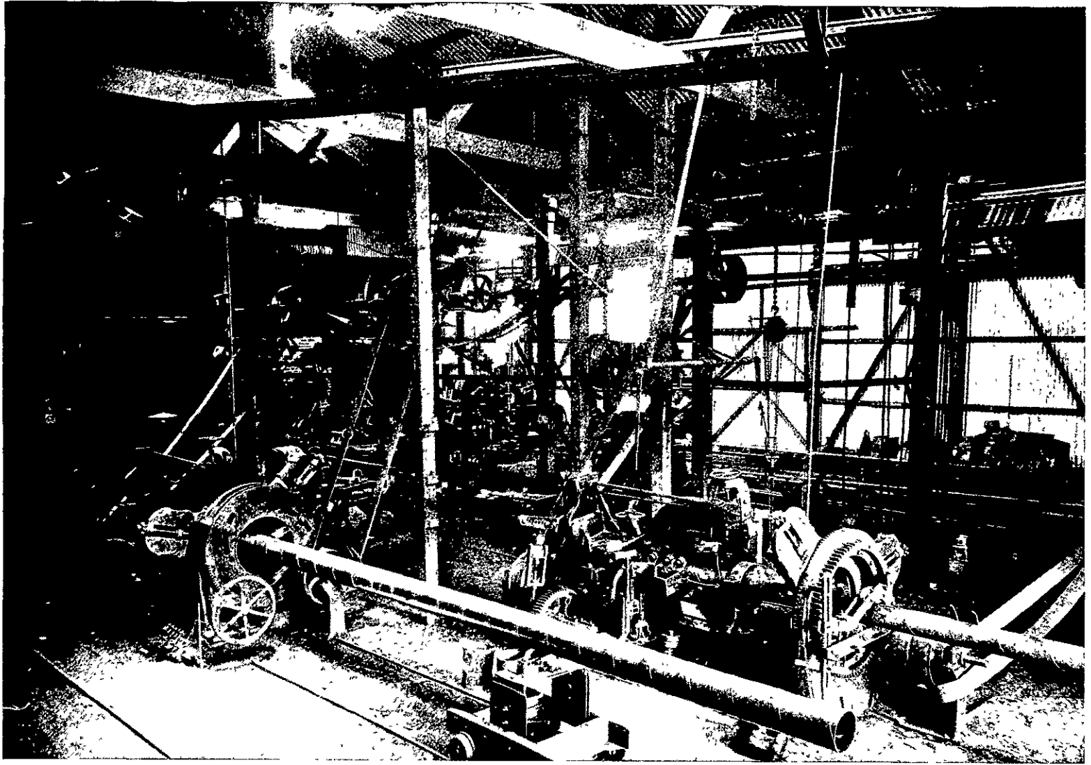
THE SPIRAL STEEL PIPE COMPANY'S WORKS: MAKING THE PIPES.
