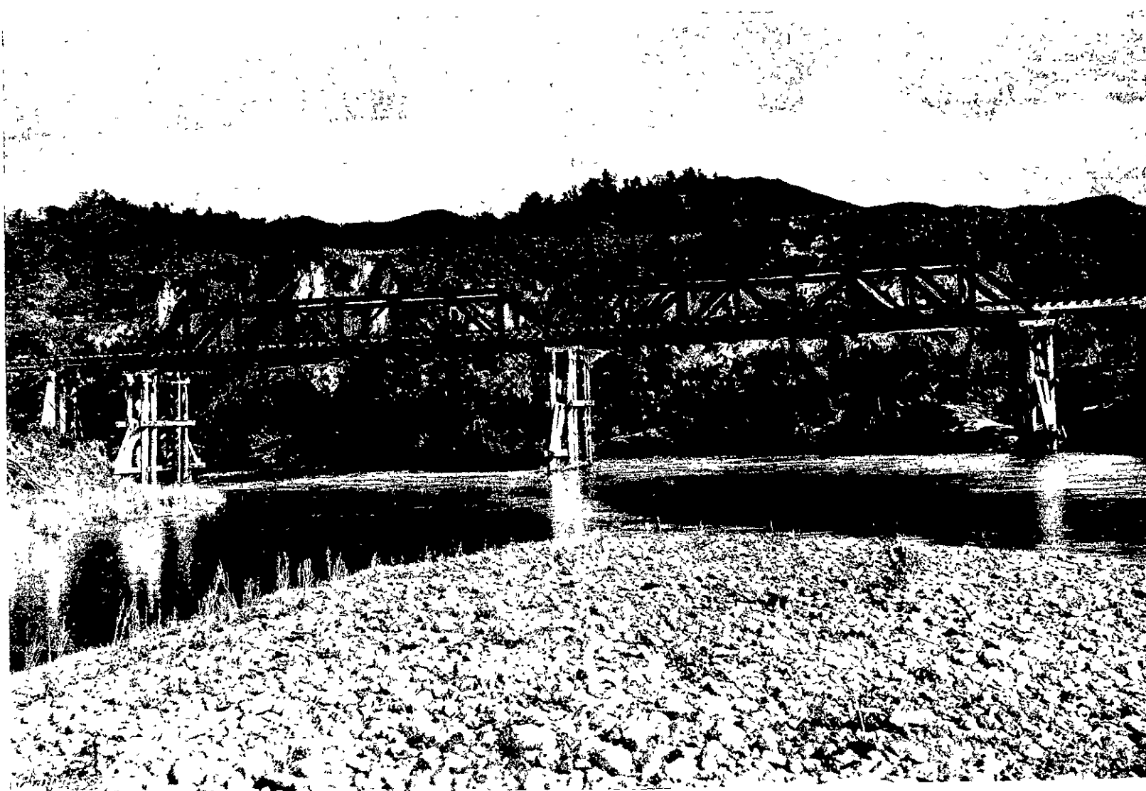
ONGARUE RIVER BRIDGE (No. 3 CROSSING). Six 20 ft. and two 80 ft. spans. Height from river bed to rail level, 30 ft.
