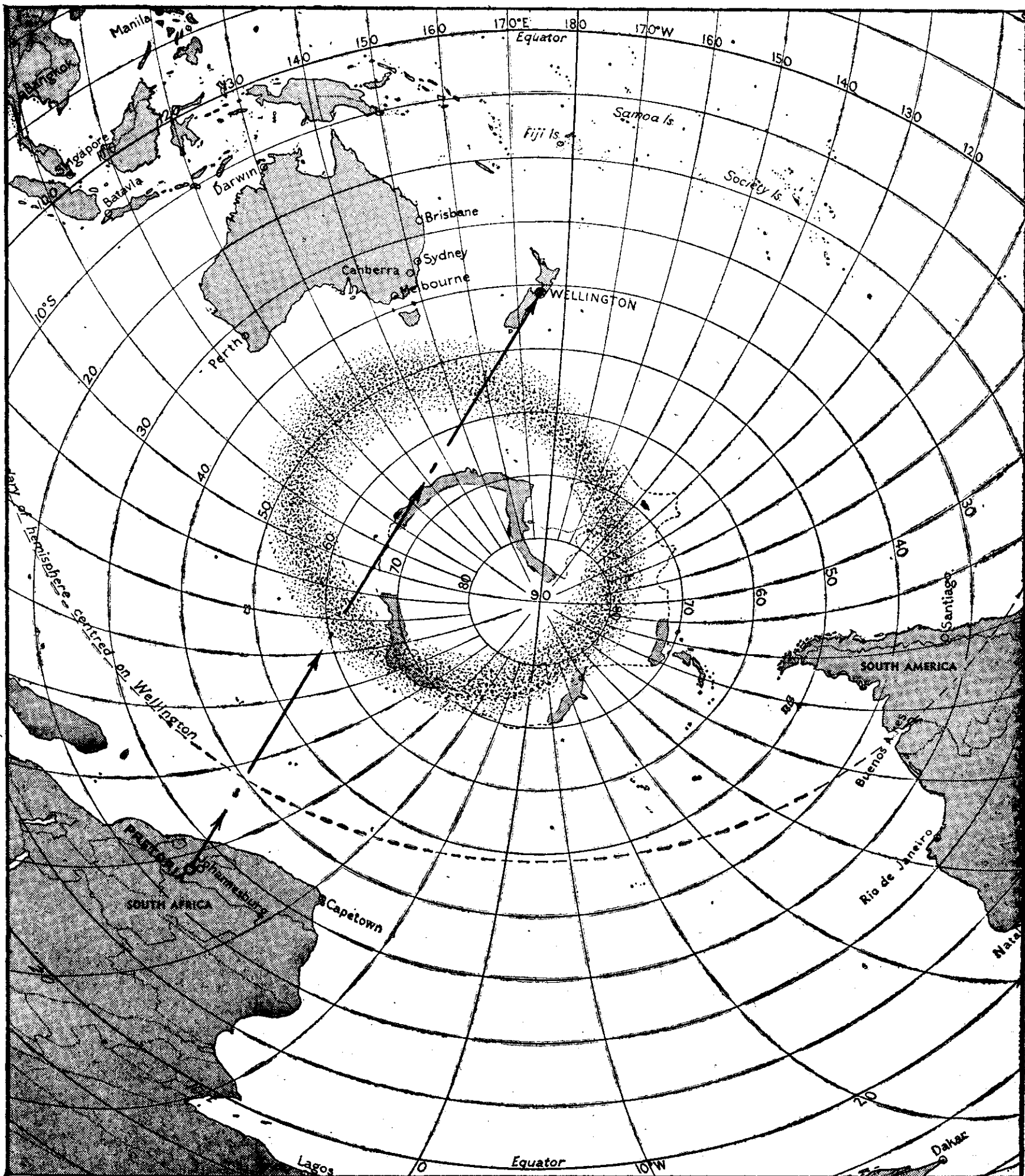
THIS MAP, part of a projection prepared by the Lands and Survey Department to show Great Circles and Azimuths from Wellington to all parts of the world, indicates the difficulties encountered in shortwave transmission from South Africa to New Zealand. The central shaded area is the Southern Auroral Zone.
