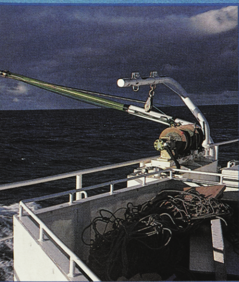
Pole at stern of longline boat. Streamers from this pole scare birds away and can reduce bait loss to birds by 69 percent. Photo: Nigel Brothers.
