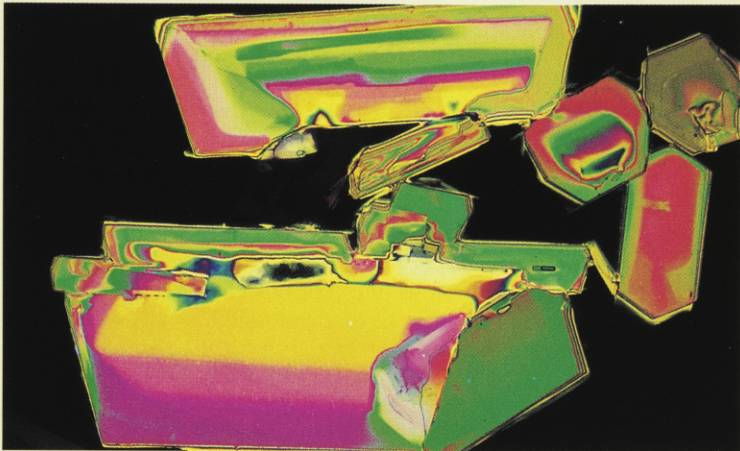
Crystals of oxalic acid
