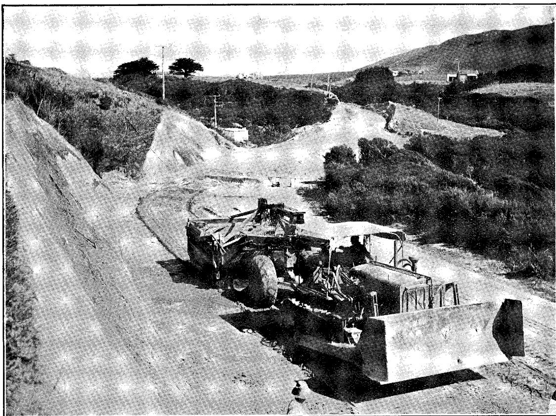
ROAD-FORMATION AND MATERIALS TRANSPORT WITH "CARRYALL," NEAR PUKERUA BAY. NOTE BULL-DOZER HEAD ON TRACTOR.
