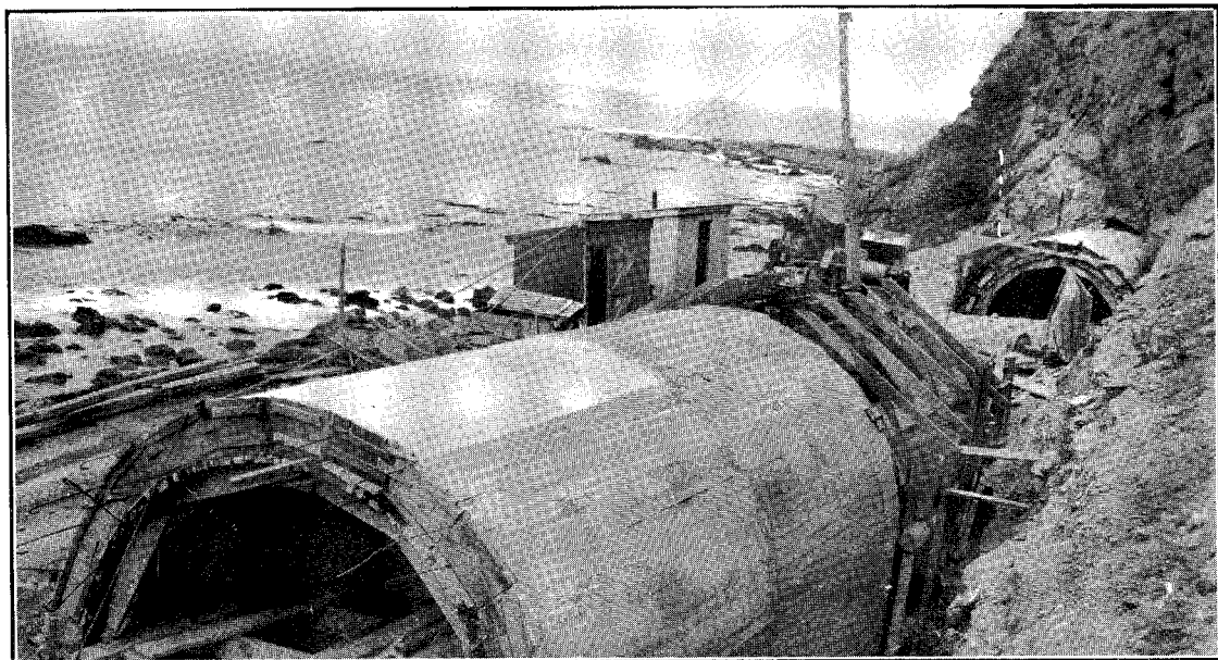
TUNNEL AT 82 M. 1 CH. LOOKING SOUTH. SPECIAL REINFORCED-CONCRETE LINING BEING BUILT PAST BAD SLIP COUNTRY.
