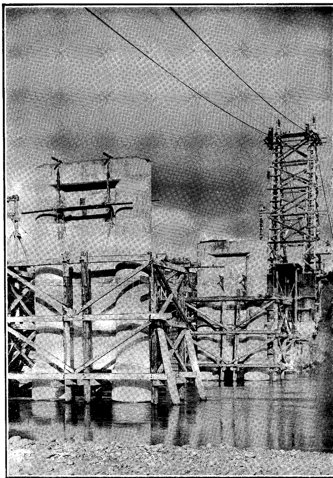
BULLER RIVER BRIDGE. PIER-CONSTRUCTION AND ERECTION CABLEWAYS.
