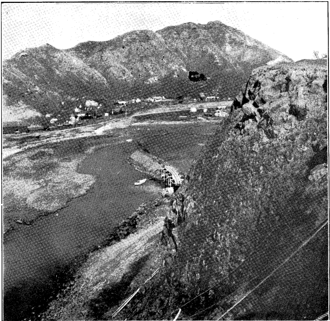
RAILWAY FORMATION, WAIKOKOPU BLUFFS. NAPIER-GISBORNE RAILWAY.
