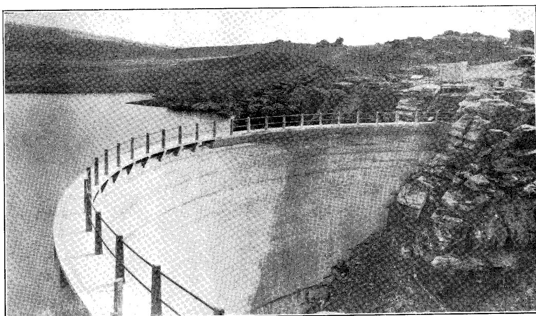
BUTCHER'S CREEK DAM. LAST CHANCE IRRIGATION SCHEME.
