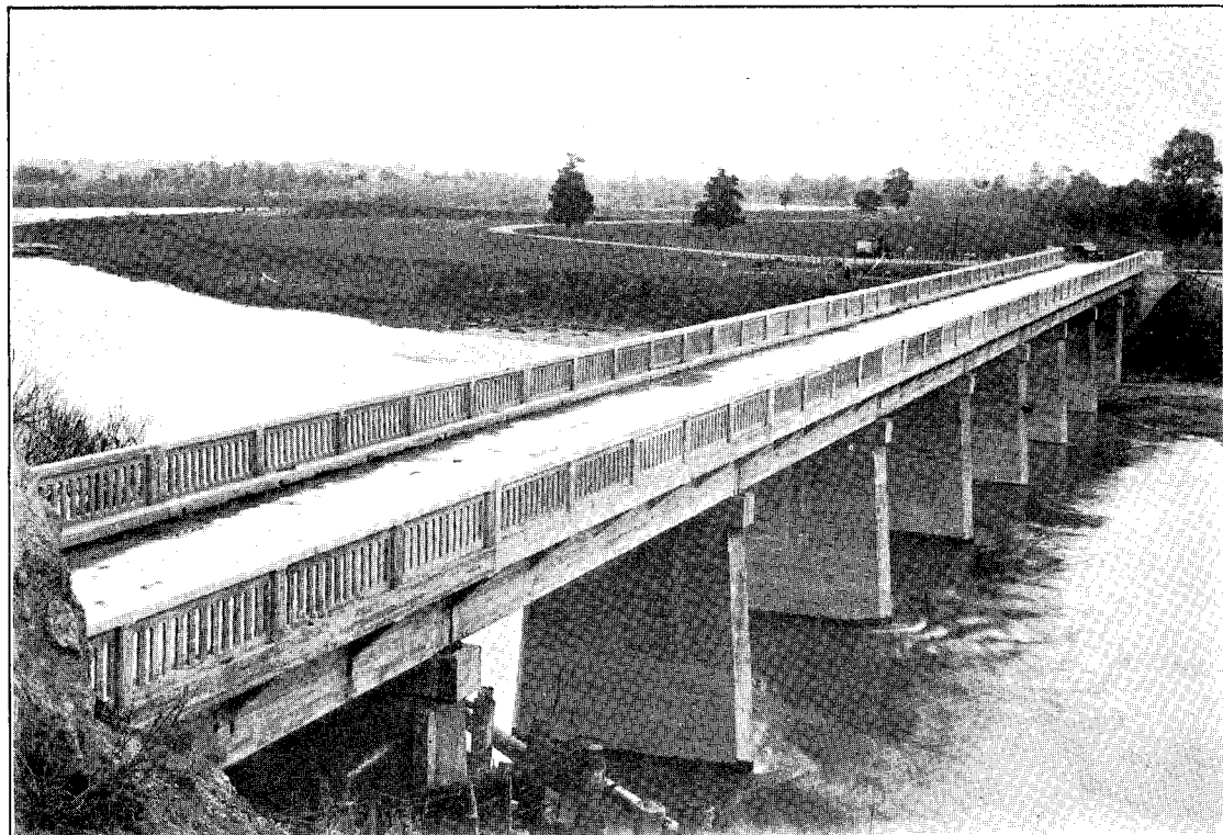
CARTERTON-GLADSTONE MAIN HIGHWAY.—KOKOTAU ROAD BRIDGE. Nine 45 ft. spans, reinforced concrete ; 18 ft. roadway.
