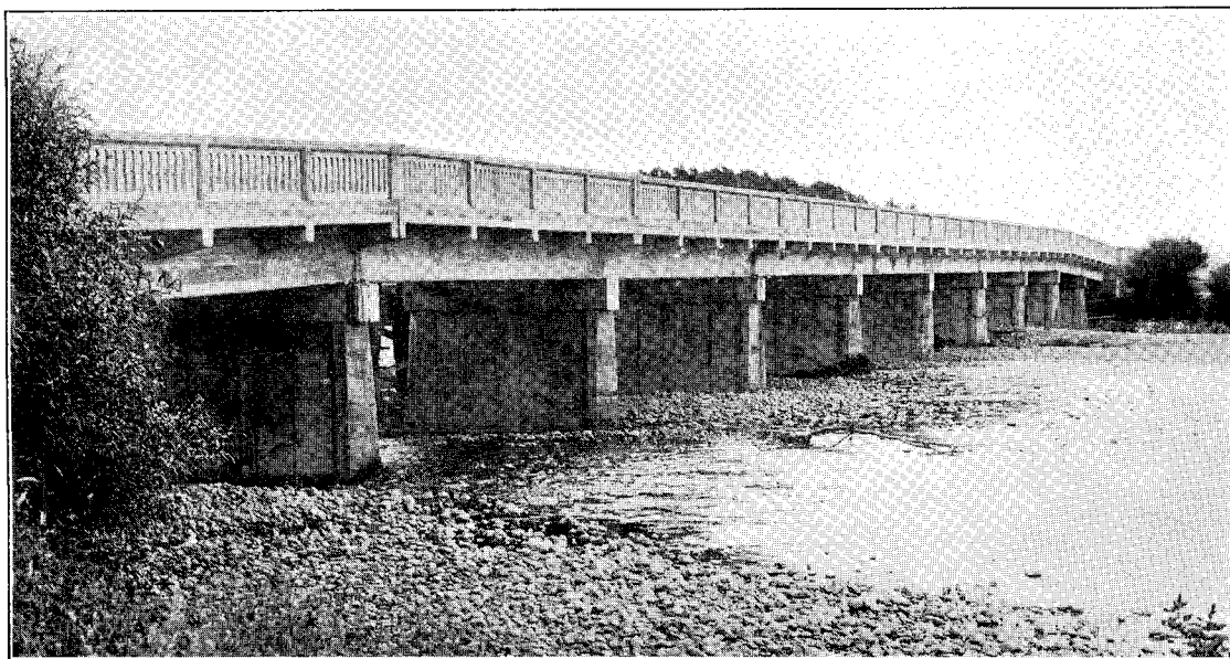
MASTERTON-TINUI MAIN HIGHWAY.—RUAMAHANGA RIVER ROAD-BRIDGE. Eleven 40 ft. spans, reinforced concrete ; 18 ft. roadway.
