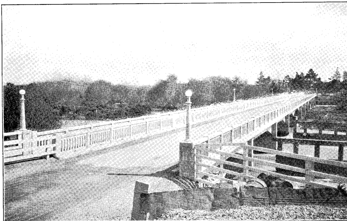
GREATFORD-WOODVILLE MAIN HIGHWAY.—AORANGI ROAD BRIDGE. Twelve 48 ft. spans, reinforced concrete ; 20 ft. roadway and 4 ft. footway.
