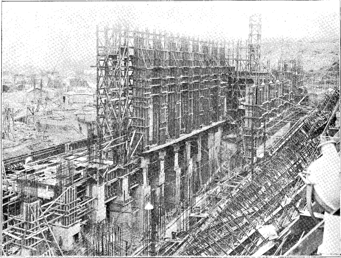
VIEW SHOWING DETAILS OF POWER-HOUSE CONSTRUCTION.
