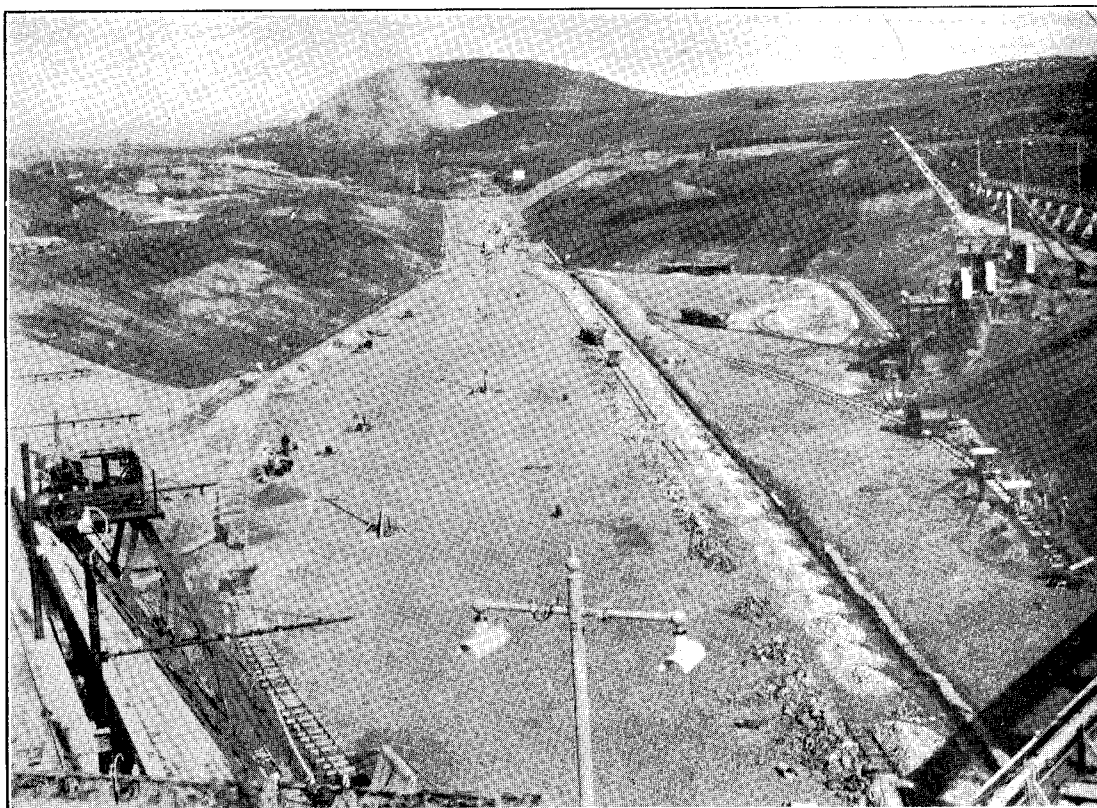
HEADRACE AND FOREBAY, LOOKING SOUTH. 5th July, 1931.
