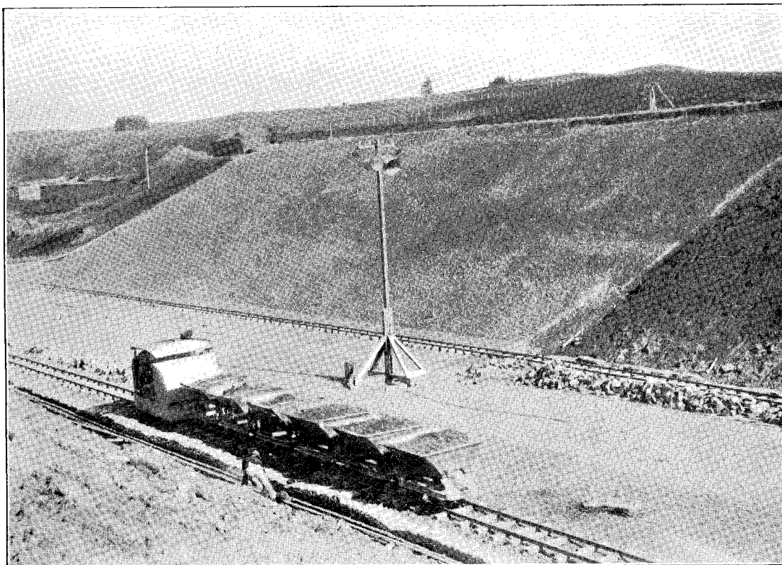
HEADRACE, SOUTH END WESTERN EMBANKMENT, SHOWING POROUS LAYER OF SHINGLE.
