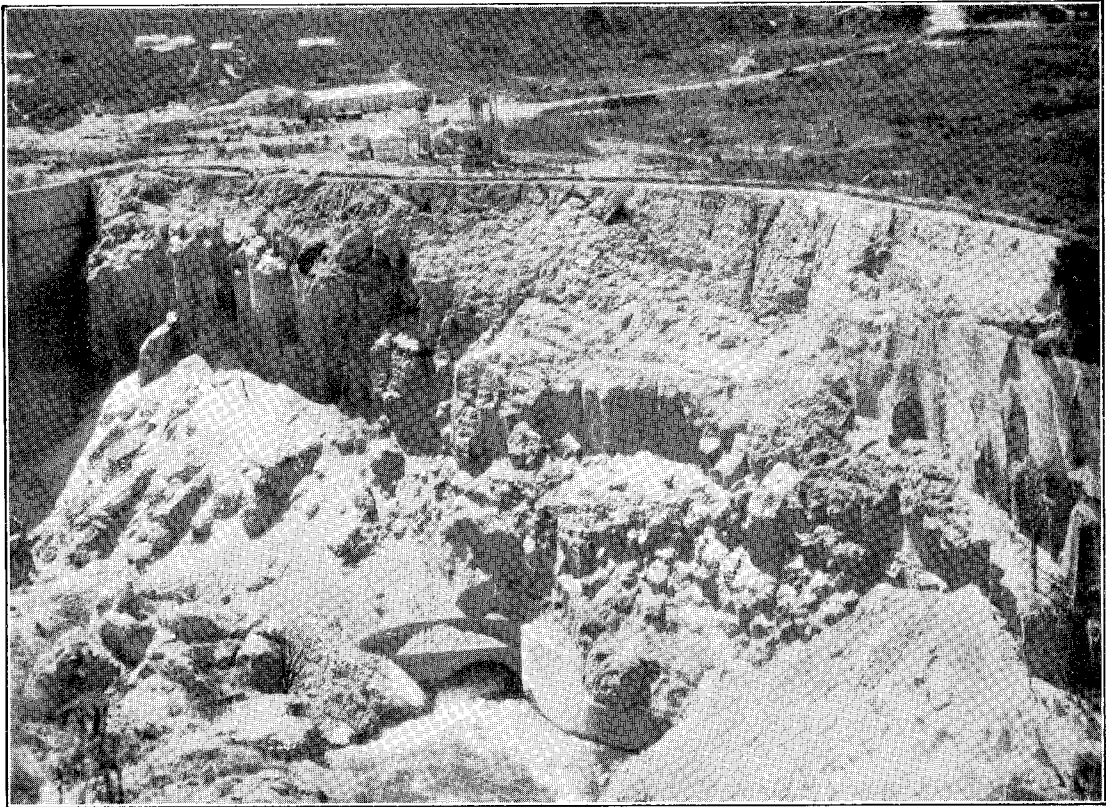
CLIFF ABOVE INTAKE OF DIVERSION TUNNEL, WITH LOOSE ROCK REMOVED.
