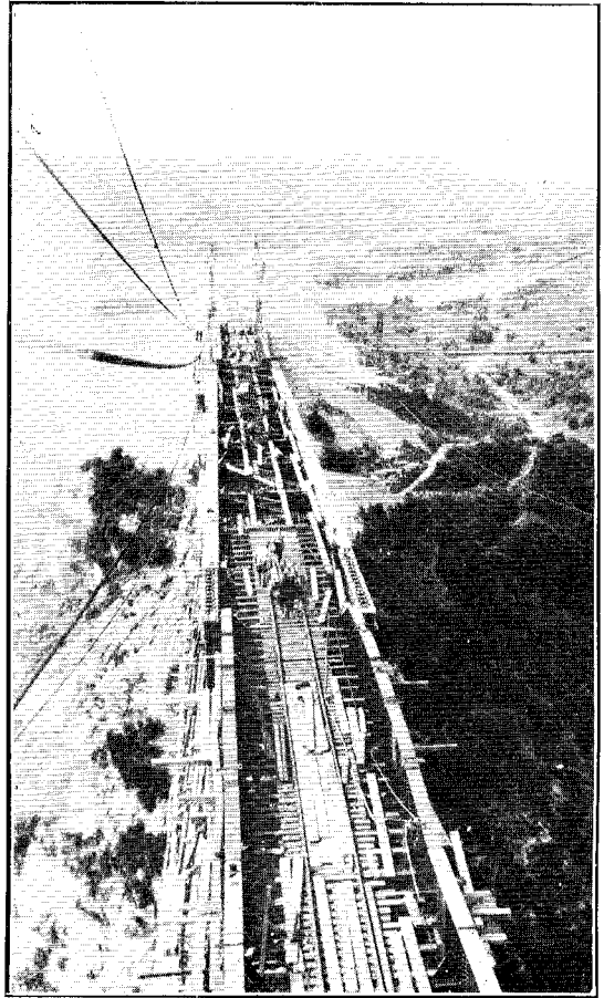
VIEWS SHOWING 250 FT. SPAN IN COURSE OF ERECTION.
