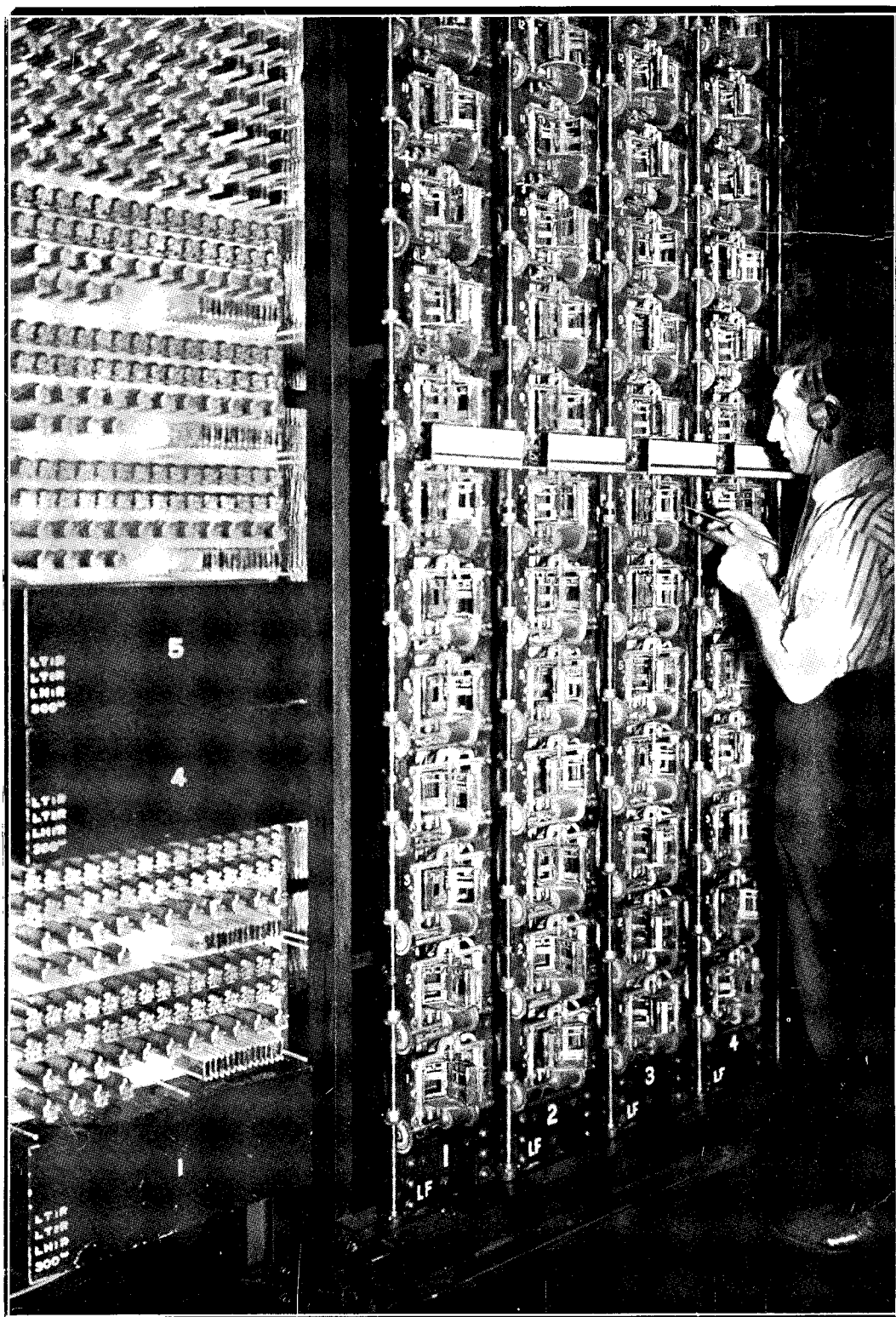
AUTOMATIC TELEPHONE EXCHANGE, WELLESLEY STREET, AUCKLAND. Small section of relays and selecting switches undergoing final adjustment.
