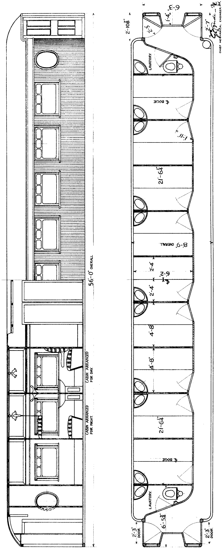
DIAGRAM OF 56 FT. SLEEPING CAR FOR 18 PASSENGERS.
