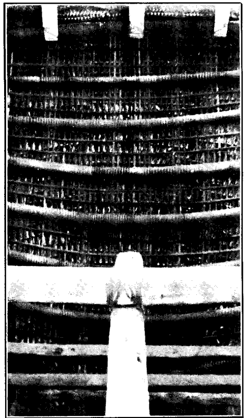
FIG. 14.—Roof of fale . No nails are used, the materials all being bound with 'afa , a string made from the fibres of the coconut-husk.
