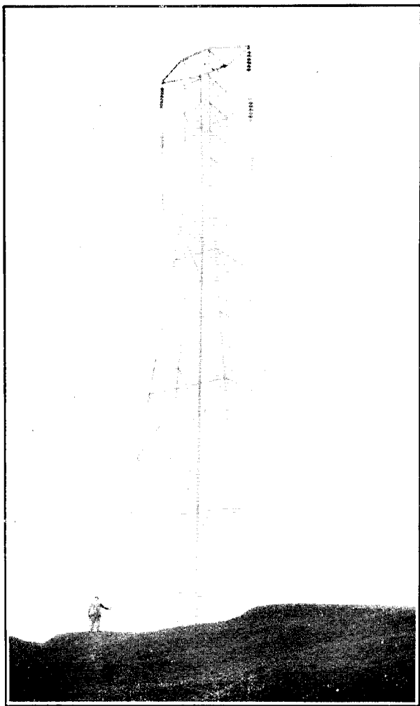
MANGAHAO HYDRO-ELECTRIC POWER PLANT: 110,000 VOLT TRANSMISSION LINE TOWERS.
