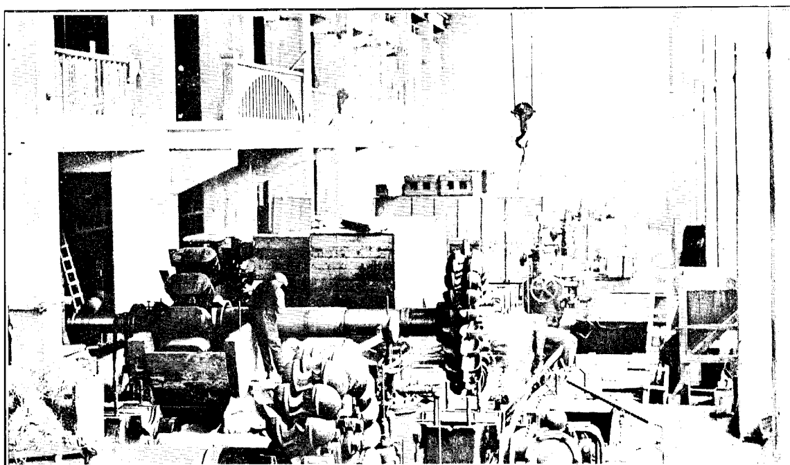
MANGAHAO HYDRO-ELECTRIC POWER PLANT: PLACING MACHINERY IN POSITION IN POWER HOUSE.
