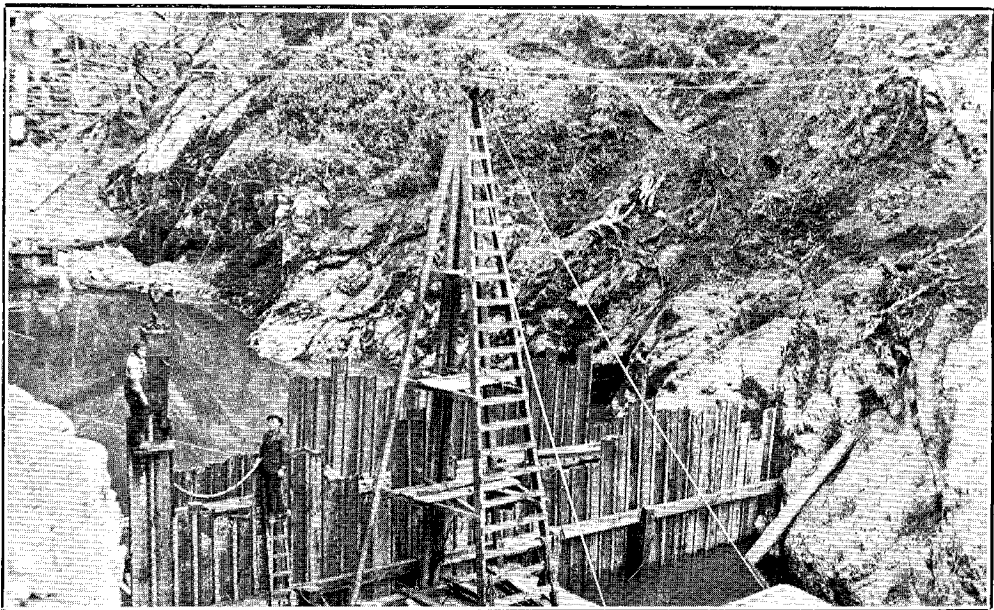
MANGAHAO HYDRO-ELECTRIC-POWER PLANT : STEEL-SHEET PILE COFFER-DAM FOR MANGAHAO DAM FOUNDATIONS.
