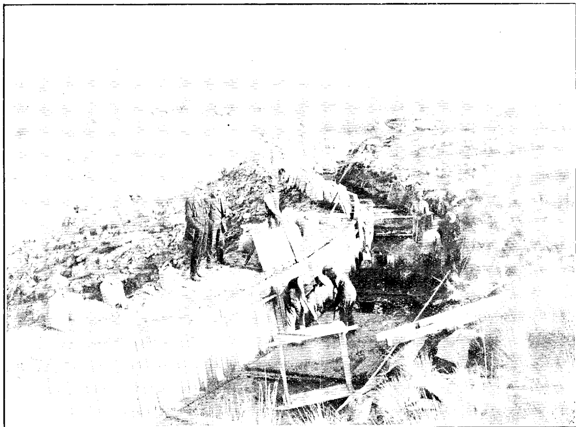
IDA VALLEY IRRIGATION. MAIN WATER RACE: VIEW SHOWING CONCRETE LINING UNDER CONSTRUCTION.
