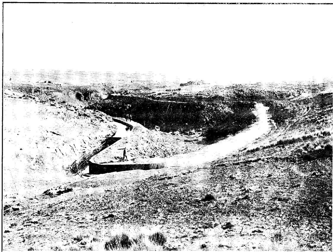
IDA VALLEY IRRIGATION. MAIN WATER RACE: VIEW SHOWING COMPLETED CONCRETE LINING.
