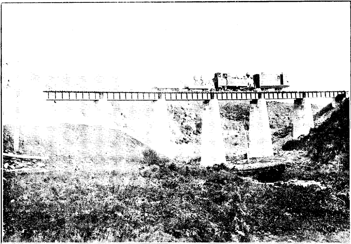
EAST COAST MAIN TRUNK RAILWAY. ATHENS SECTION : GENERAL VIEW OF BRIDGE AT 6 M. 60 CH.
