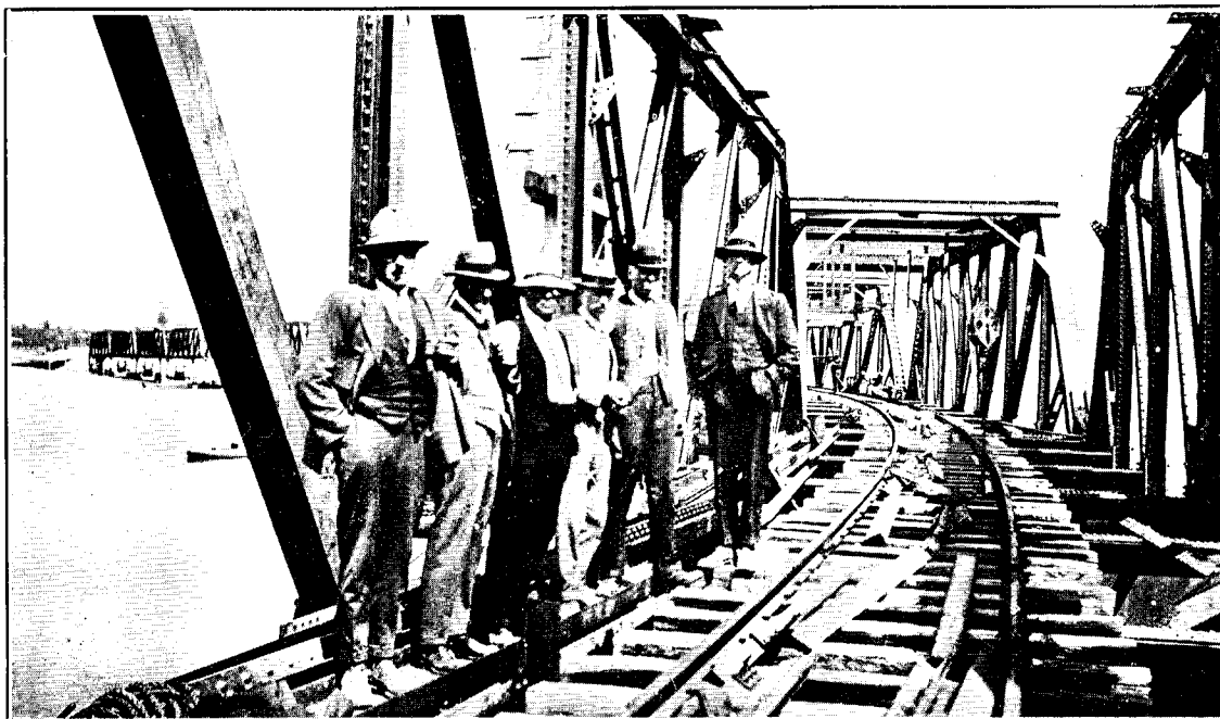
EAST COAST MAIN TRUNK RAILWAY. TAURANGA HARBOUR BRIDGE: VIEW SHOWING 105 FT. SPAN ON CURVE.
