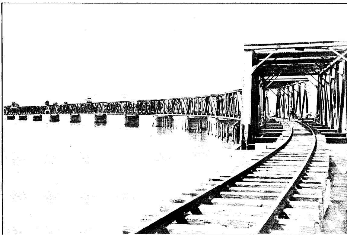
EAST COAST MAIN TRUNK RAILWAY. TAURANGA HARBOUR BRIDGE: GENERAL VIEW OF BRIDGE FROM TAURANGA END.
