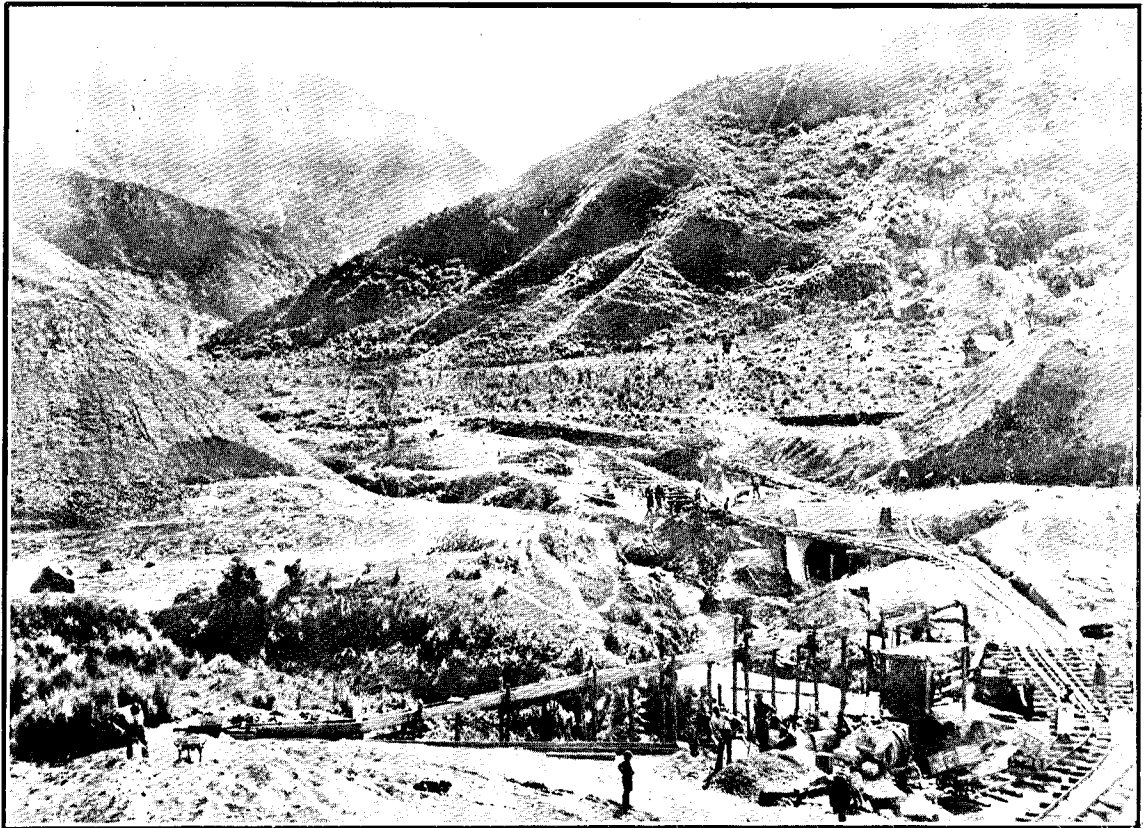
Wairoa Waikopu Railway: 12 ft. Culvert at 22 Miles 30 Chains, showing Gravel-washing Plant and Filling-in Progress.
