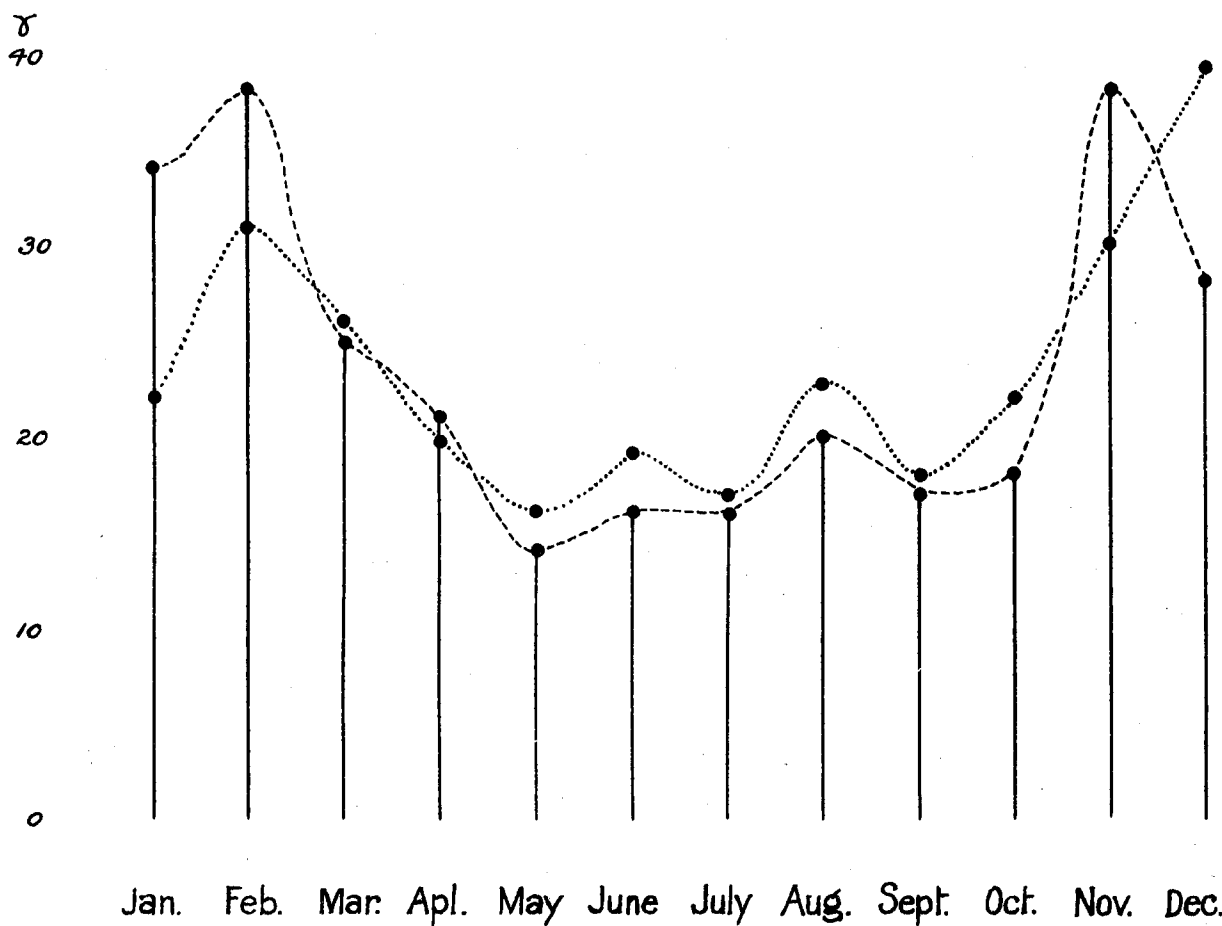
Curve showing Mean diurnal Range of Horizontal Force at Christchurch for 1914 thus----- for 1913 thus.....
