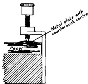
— Detail of — — Paper Clamp —
