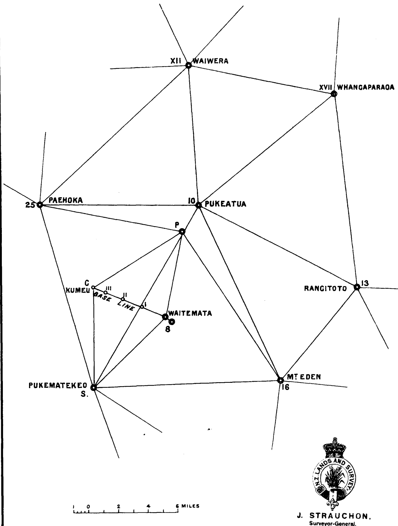
WAIKEMATA BASE LINE.—Fig.1.
