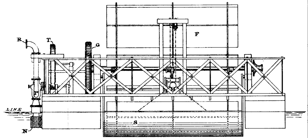
— END ELEVATION. —
