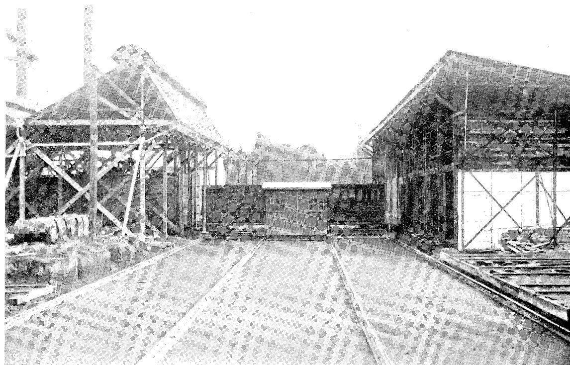
ELECTRIC TRAVERSER AND BINNS, POWELL WOOD PROCESS WORKS, RANGATAUA.
