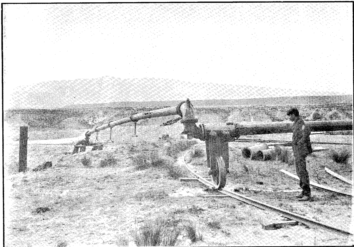
SWIVELLING ARRANGEMENT FOR SUPPLYING WATER TO WORK GOLDEN BEACH DREDGE, ALEXANDRA.
