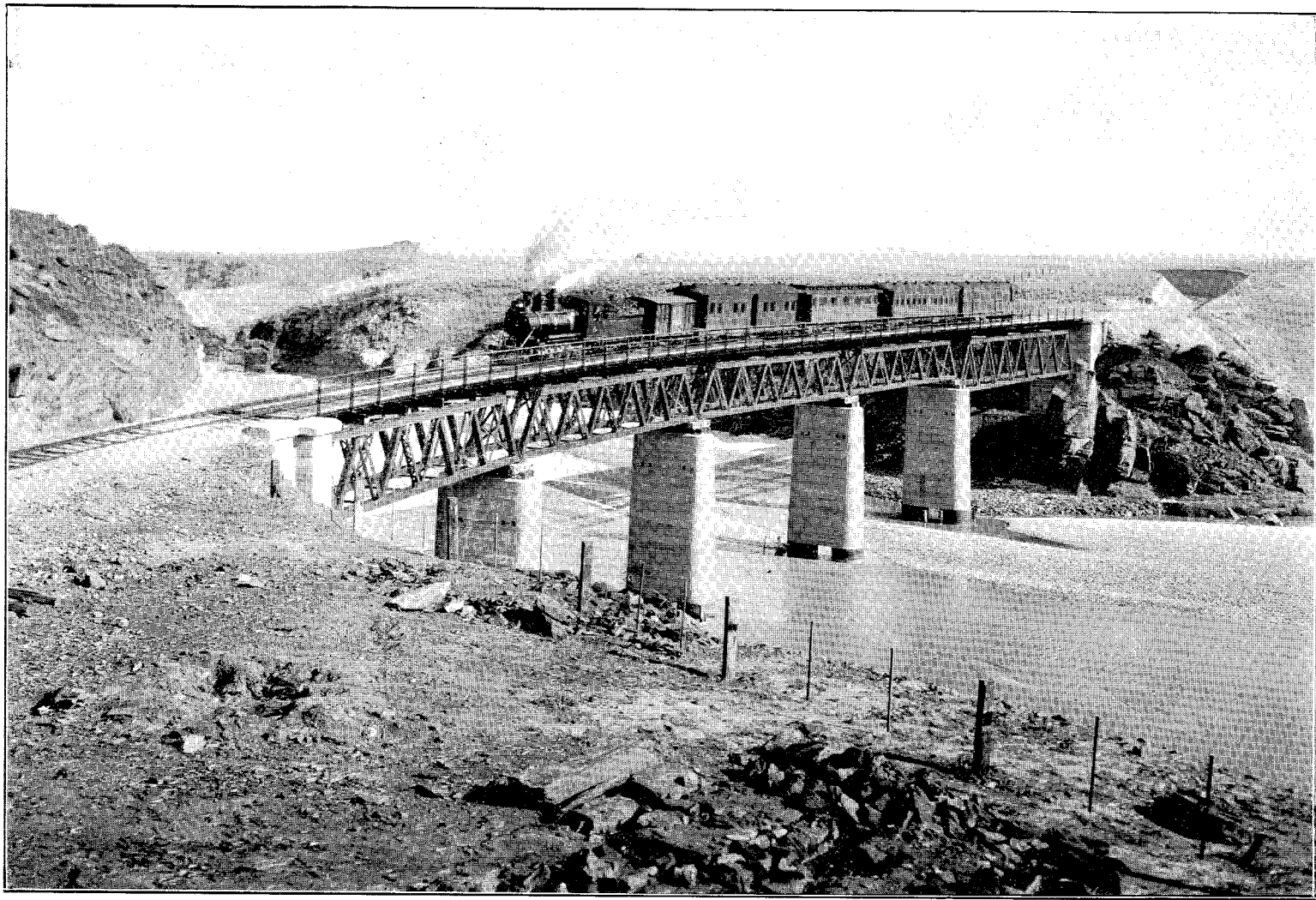
OTAGO CENTRAL RAILWAY. BRIDGE OVER MANUHERIKIA RIVER, FIRST CROSSING. ONE 100 FT. AND FOUR 66 FT. STEEL GIRDER SPANS ON CYLINDER AND CONCRETE PIERS; LENGTH OVER ALL, 368 FT.; HEIGHT, RIVER-BED TO RAIL-LEVEL, 50 FT.
