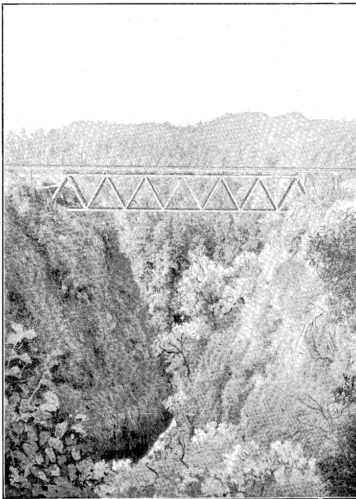
NORTH ISLAND MAIN TRUNK RAILWAY. BRIDGE OVER TOI CREEK, 37 MILES 54 CHAINS FROM MARTON JUNCTION; ONE STEEL GIRDER SPAN OF 156 FT., TWO TIMBER SPANS OF 20 FT., AND TWO 11 FT.; 187 FT. FROM CREEK-BED TO RAIL-LEVEL.
