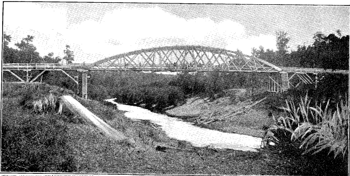
Mangakahia Bridge
