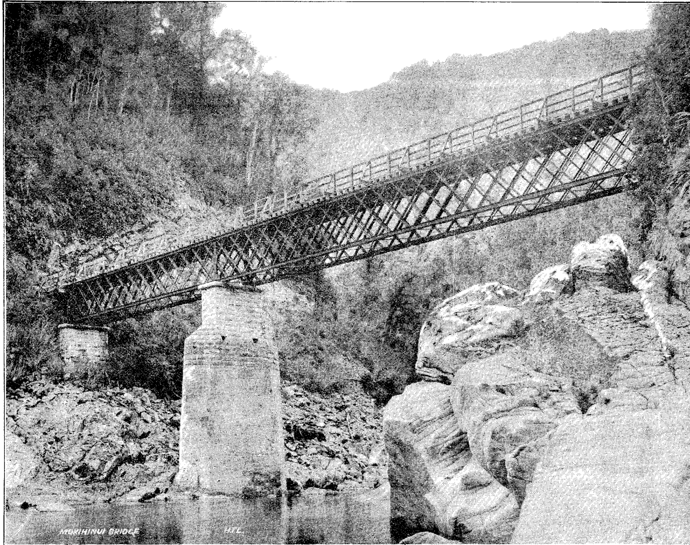
Mokihinui Gorge Road Bridge: One span of 144 ft., and one of 84 ft.
