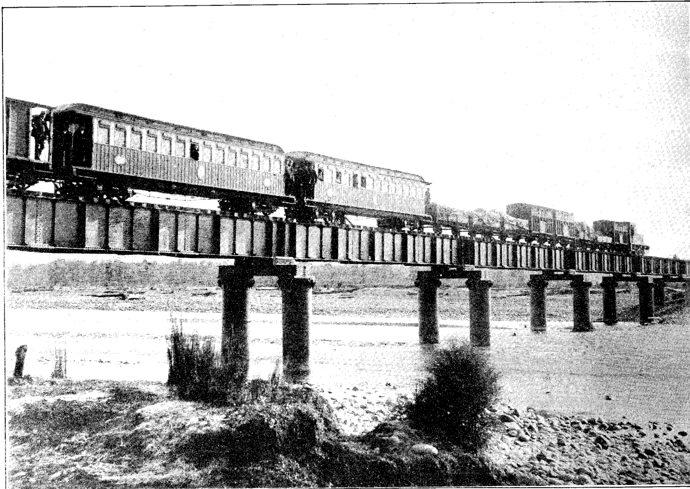
Midland Railway, Bridge over Little Grey River: Ten spans of 66 ft., and three of 11 ft.; total length of cylinders, 33 ft.
