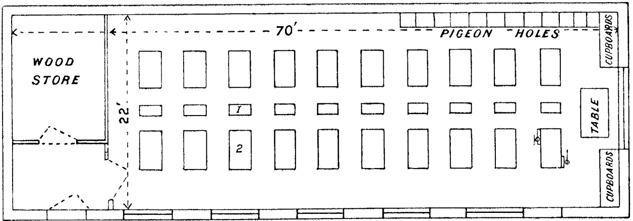
XIII.—PLAN OF CLASS-ROOM FOR MANUAL INSTRUCTION IN WOOD.
