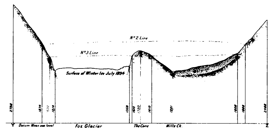
Cross section on Line yz.
