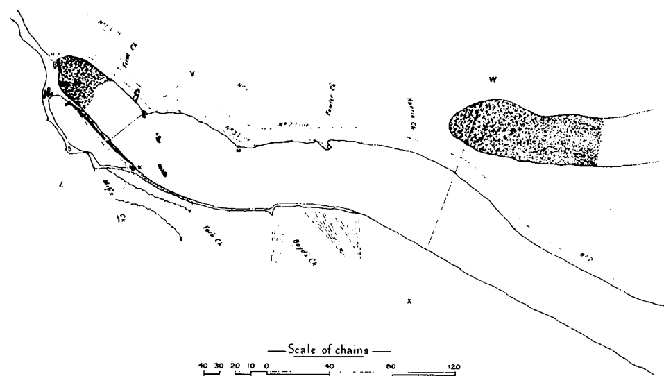
— Diagram of — — Flow of Glacier. —
