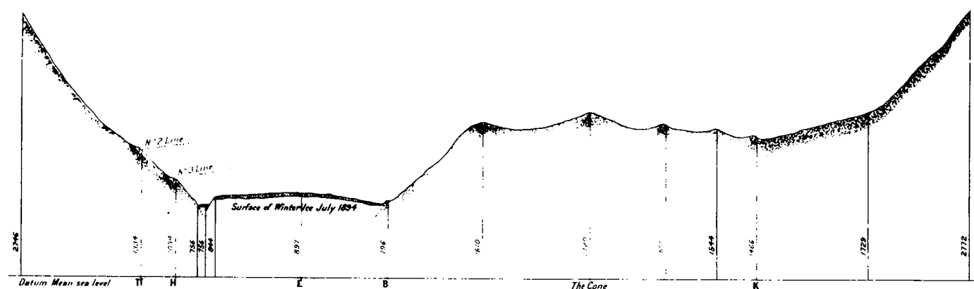
Section on Lines π.H.E.B.K.
