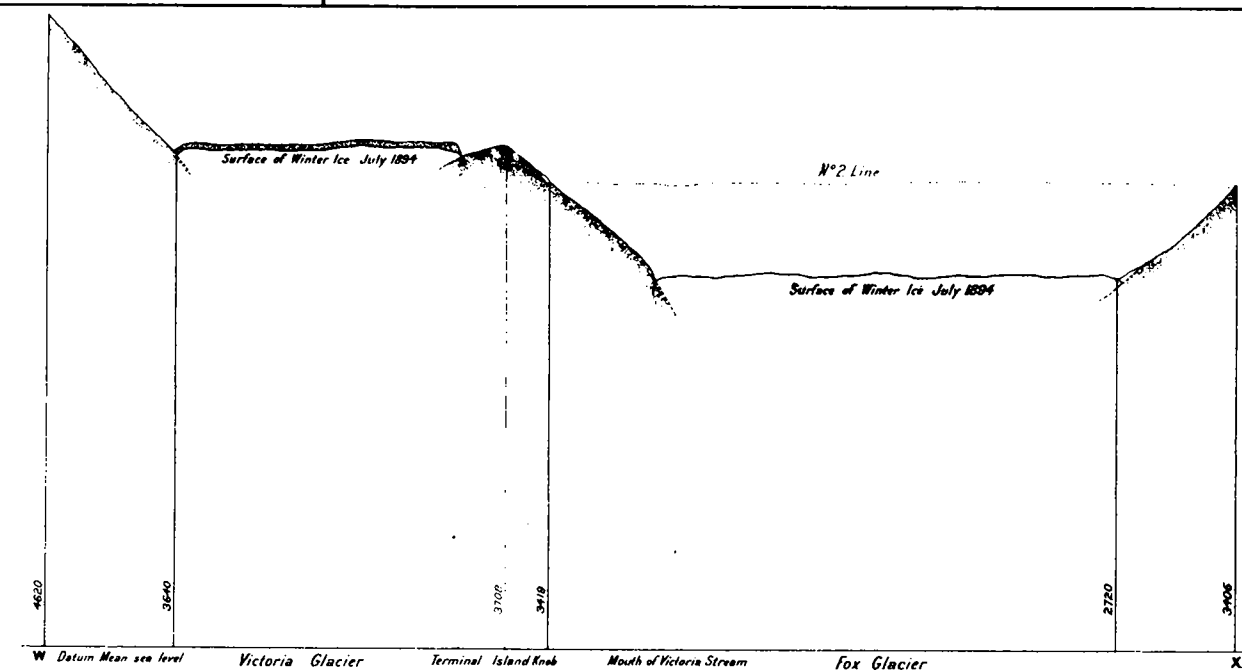
Cross section on Line wx.
