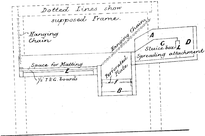
— Section through Y.Z. —
