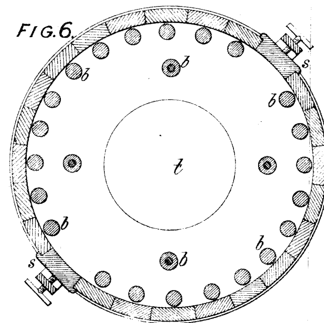
PLAN SHEWING CASSELL'S CHLORINATING PROCESS To Illustrate Report of H. A. Gordon, Inspecting Engineer.
