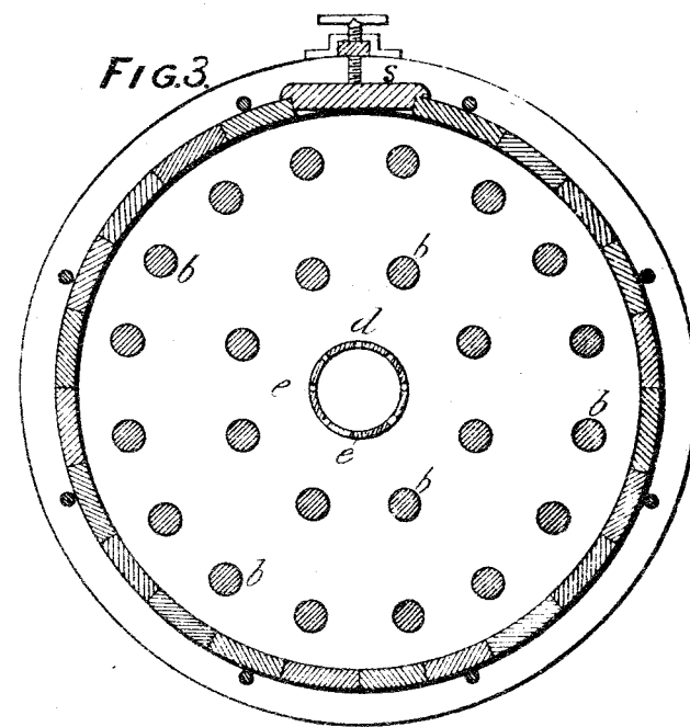
PLAN SHEWING CASSELL'S CHLORINATING PROCESS To Illustrate Report of H. A. Gordon, Inspecting Engineer.
