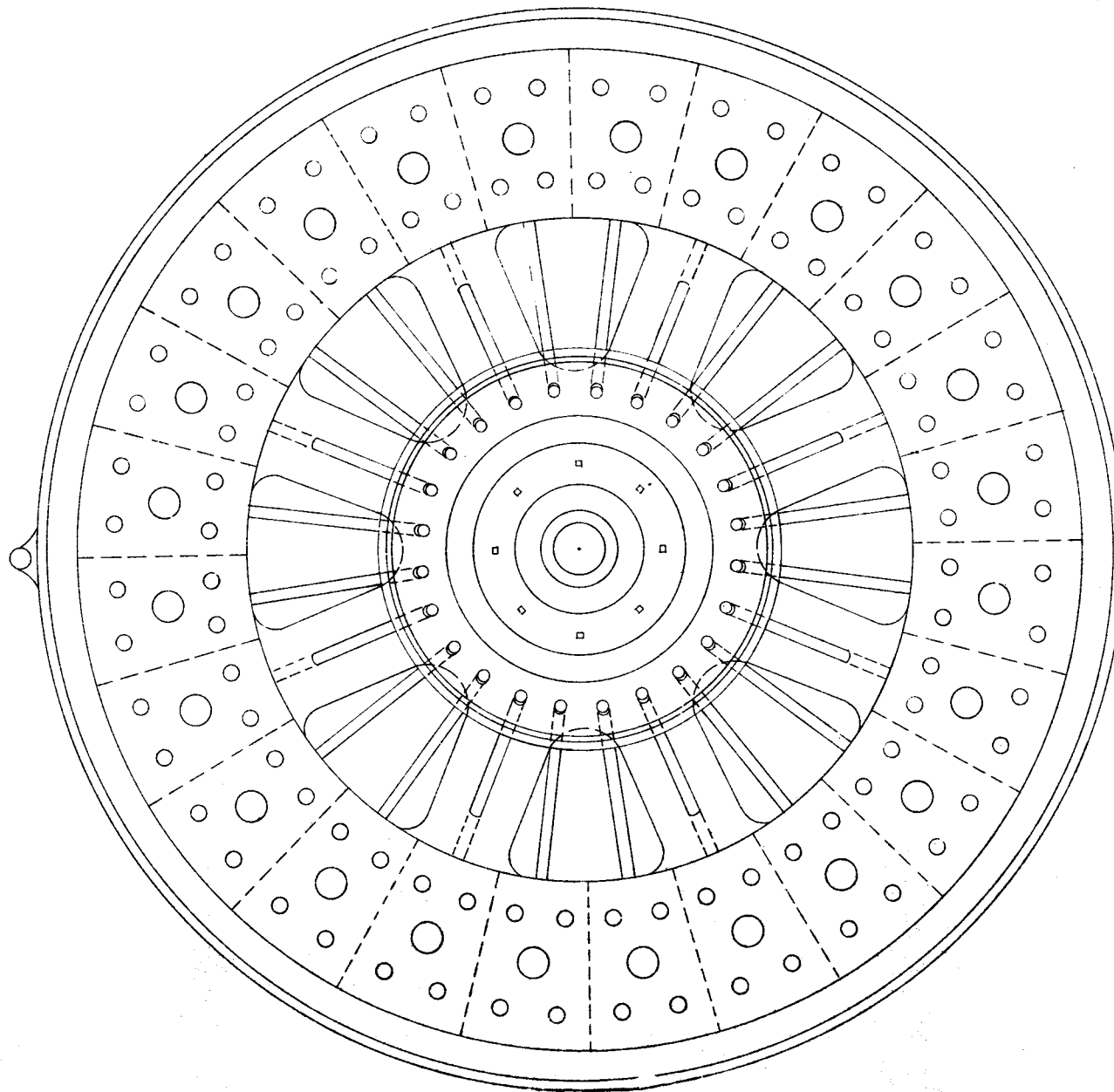
CLIMO AND BAWDEN'S GRINDING AND AMALGAMATING PAN.
