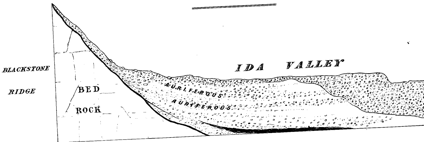
AURIFEROUS LAKE AND RIVER DRIFT, WOOLSHED DIGGINGS.
