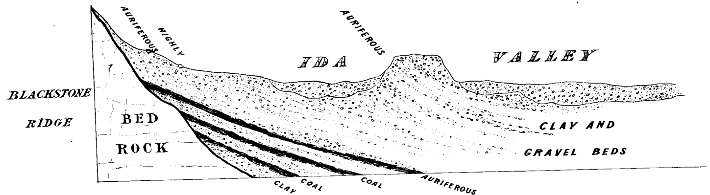
AURIFEROUS LAKE DEPOSIT, HILL'S CREEK.
